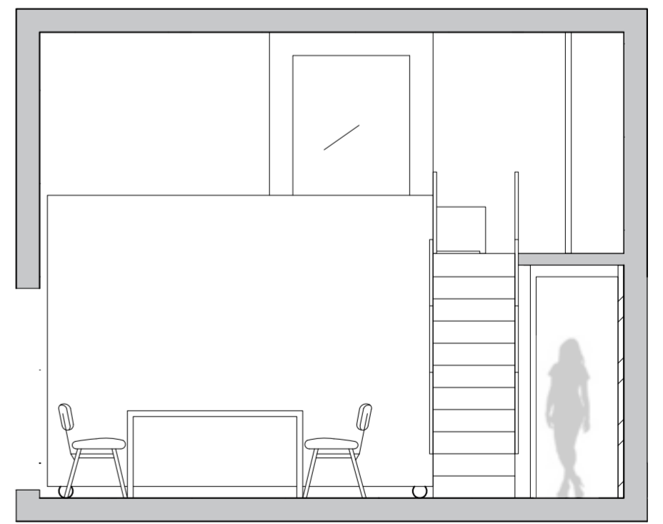
CROSS SECTION BB'
